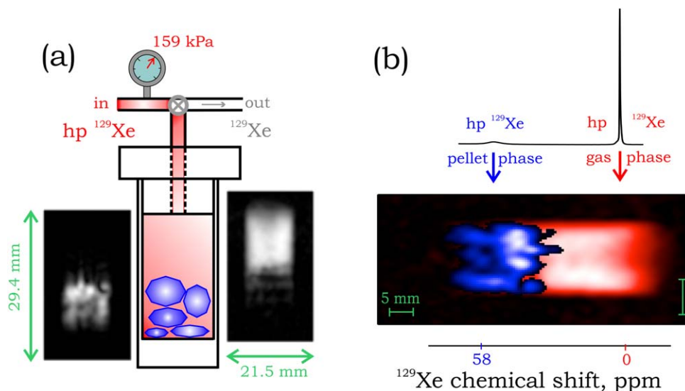
Figure 1. (a) The outline of the pellet sample holder. The sample container is evacuated and hp ^{129}\text{Xe} is delivered through the valve as shown. Pressure in the sample container is equalized to 159 kPa after the gas delivery. The images shown depict hp ^{129}\text{Xe} in the pellet phase (left) and in the gas phase (right); (b) ^{129}\text{Xe} 1-D spectrum of xenon gas in the pellet sample. The chemical shift separation between gas and the pellet phase is 58 ppm. A composite image combined from the images acquired at the pellet phase frequency (blue) and at the gas-phase frequency (red) is also shown. Please note the match in image boundaries at the interface between the gas and pellet phases.
